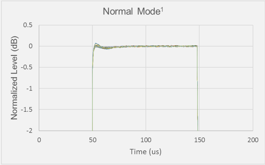
1. Measured with a 500 kHz IF bandwidth, no averaging (Average Type = Point). With 100 us pulse width setting. 50 usec/div.
